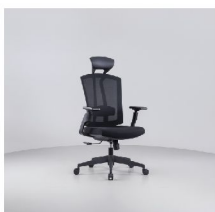
APW-F008-1-TIGRA-A-BLA-BLA D600*W690*H(1165-1260)mm (+/-20)
